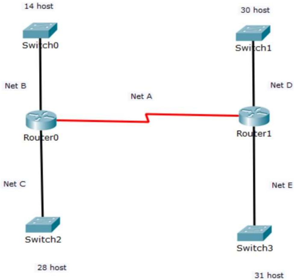
Figure 0-2 Network topology
